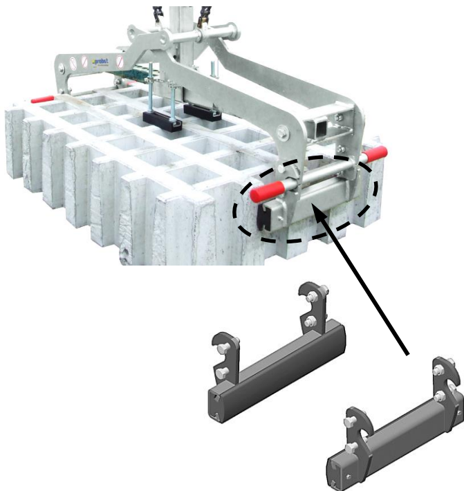
FTZ-MULTI-15 with grippers WB-SQ (for ashlar rocks) (43100941)
