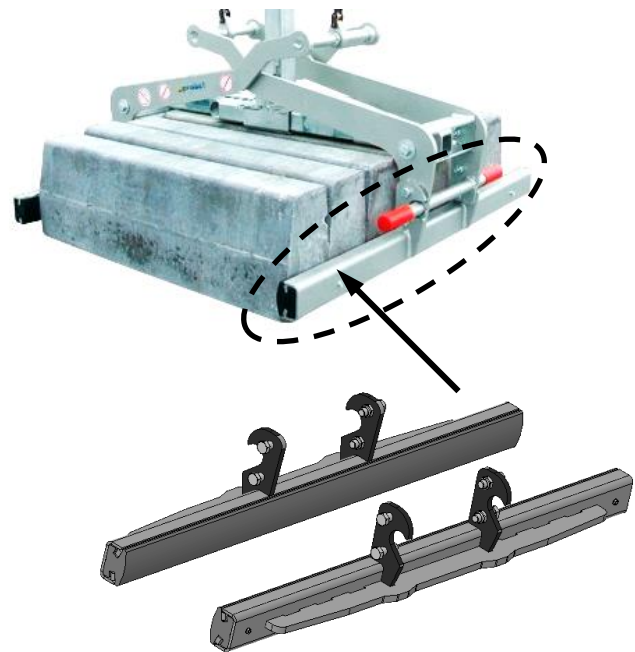
FTZ-MULTI-15 with grippers WB-G-120 (43100943)
