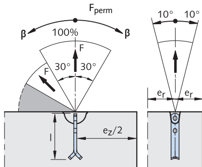
Spread anchor in beams and walls – with reinforcement subjected to load (load class 5,0–26,0)
