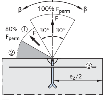
Lifting TPA-FE
