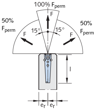
TPA-FE, tilt-up
