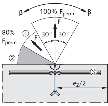
Lifting TPA-FA
