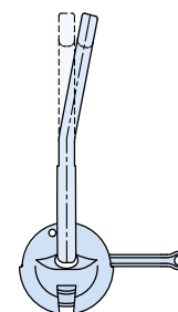
Figure: Significant bending of the shackle caused by misuse of a TPA Ring clutch
