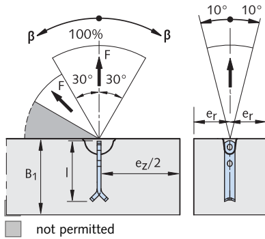
Spread anchor in beams and walls – no special reinforcement requirements (load class 5,0-26,0)
