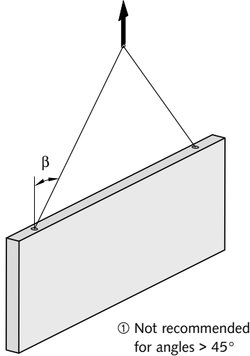
Diagonal load \beta : 10^\circ to 60^\circ ①
