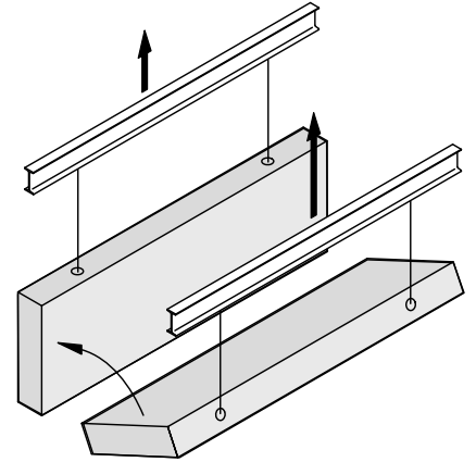
Tilt-up \gamma : 90^\circ
